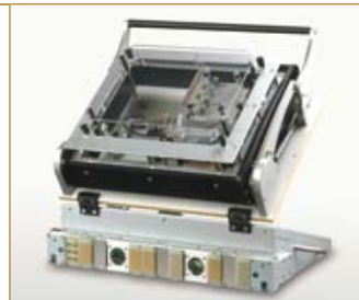
Customized Interface
