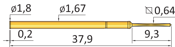
CR 100-3-05 wire wrap vacuum-sealed
