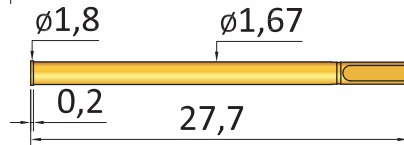
CR 100-2-05 solder cup
