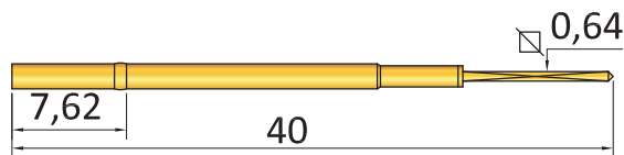
CR 100-3V wire wrap vacuum-sealed
