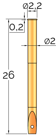
CR 112 - 0 solder cup
