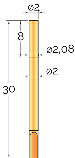
CR 112 - 2G8 solder cup
