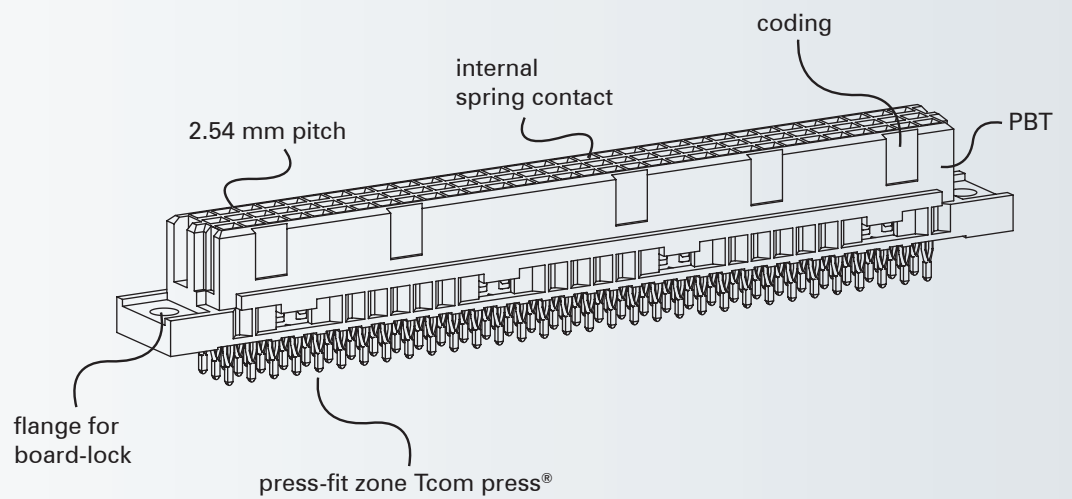
Female Connector Type C
