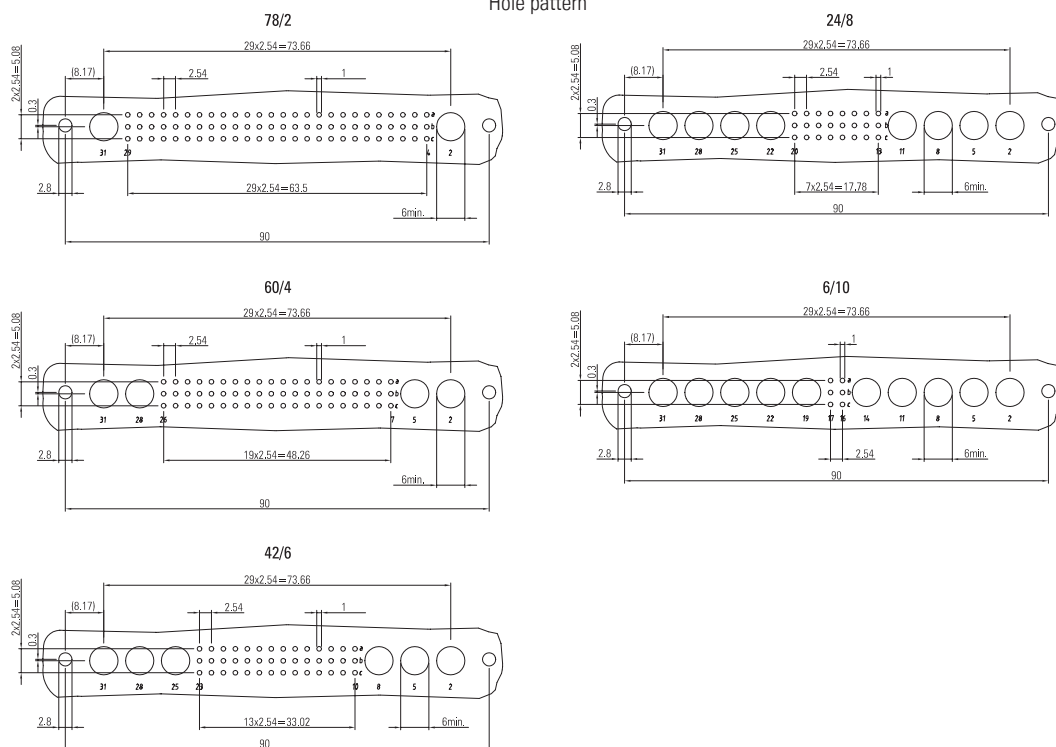
Hole pattern
