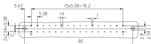
Hole pattern
